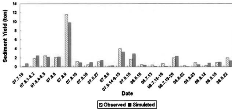
Fig. 17. Comparison of simulated and measured sediment yield from study watershed.
