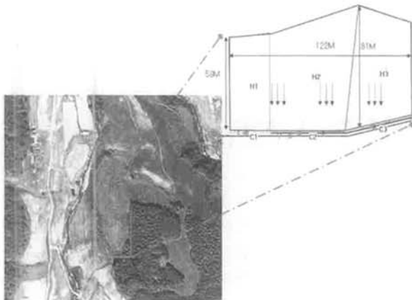
Fig. 14. Watershed configuration of the study watershed.
