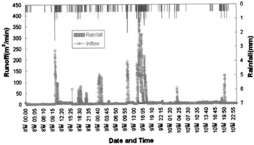
Fig. 4. Runoff and Rainfall per minute (Hyun et al., 2008).
