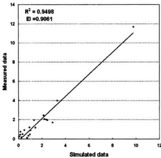
Fig. 18. R 2 and Nash-Sutcliffe of sediment estimation.
