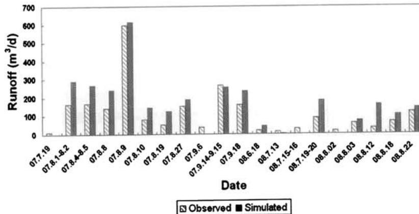
Fig. 15. Comparison of simulated and measured runoff volume from study watershed.
