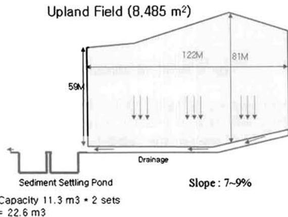
Fig. 2. Sediment settling pond (Hyun et al., 2008).
